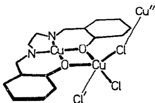
Fig. 10. Structure of \text{Cu}(\text{salen})\text{CuCl}_2 .
